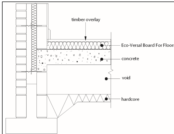
Figure 3 Ground-bearing concrete — slab overlay
