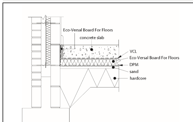
Figure 4 Suspended concrete ground floor — timber overlay
