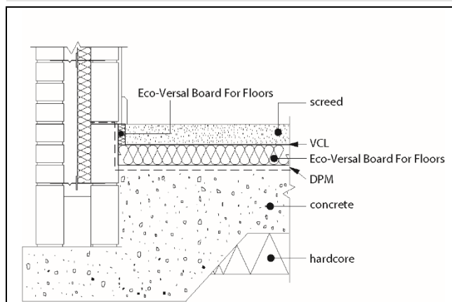
Figure 1 Ground-bearing concrete floor — screed overlay
