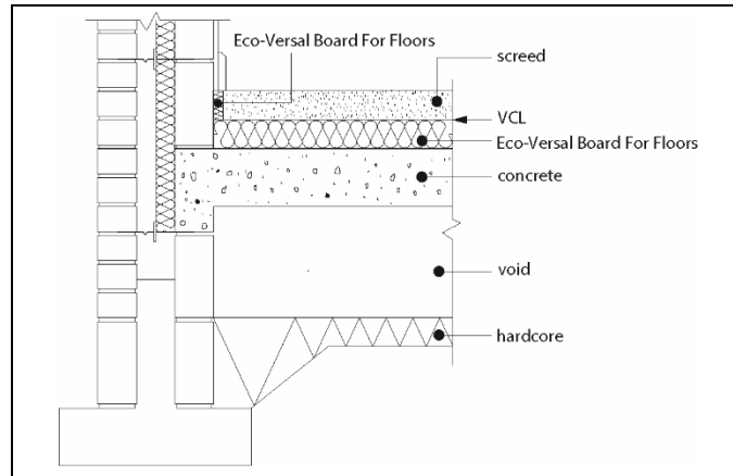
Figure 2 Suspended concrete ground floor — screed overlay
